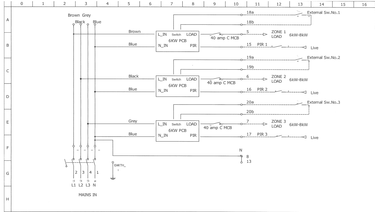
Wiring diagram for 18kW, 24kW & 27kW controllers.
